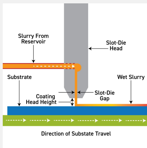
FIGURE 1. The Slot Die coating process relies on the precise control to the two distinct gaps. The first, a Slot Die Gap, is the gap between the two halves of the Slot Die Head. This separation forms the path used to deliver the Slurry to the substrate. The second gap is the Coating Head Height which is the dimension between the Slot Die Head and the Substrate.
