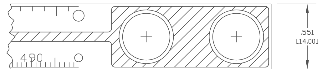
DETAIL A SCALE 2:1
