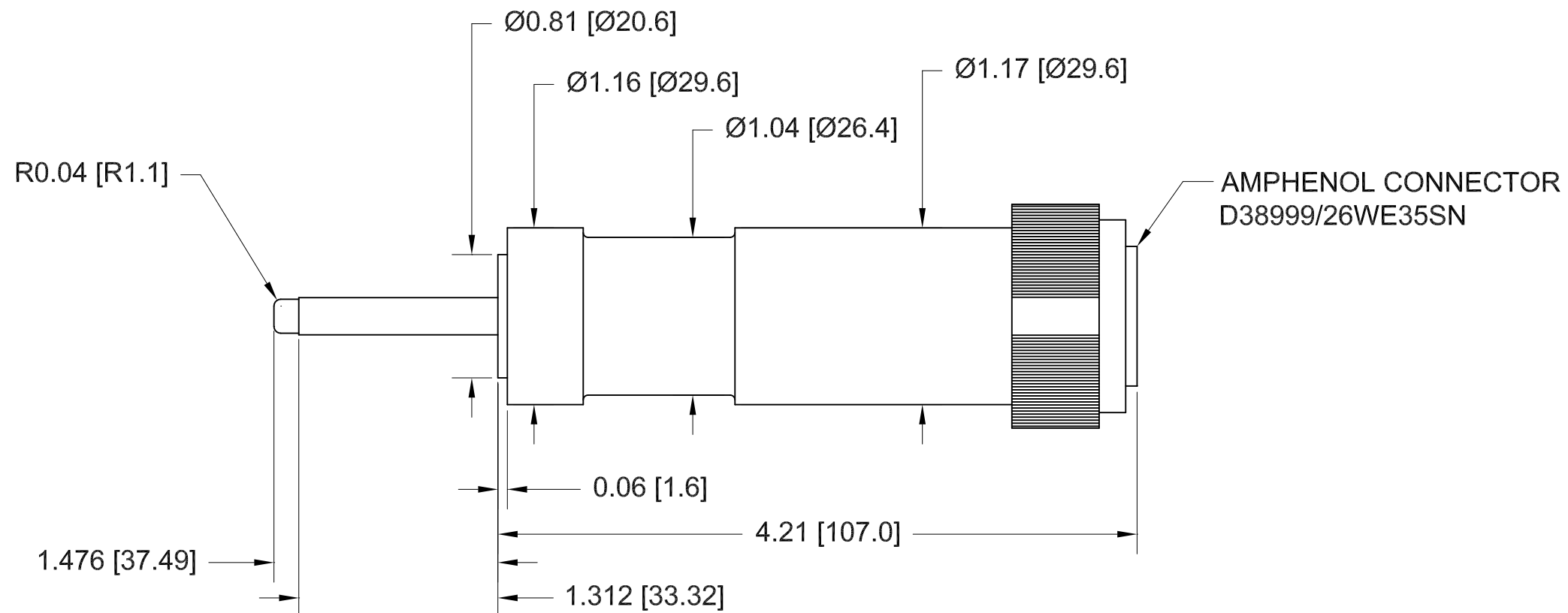
PROBE HANDLE CONFIGURATION
